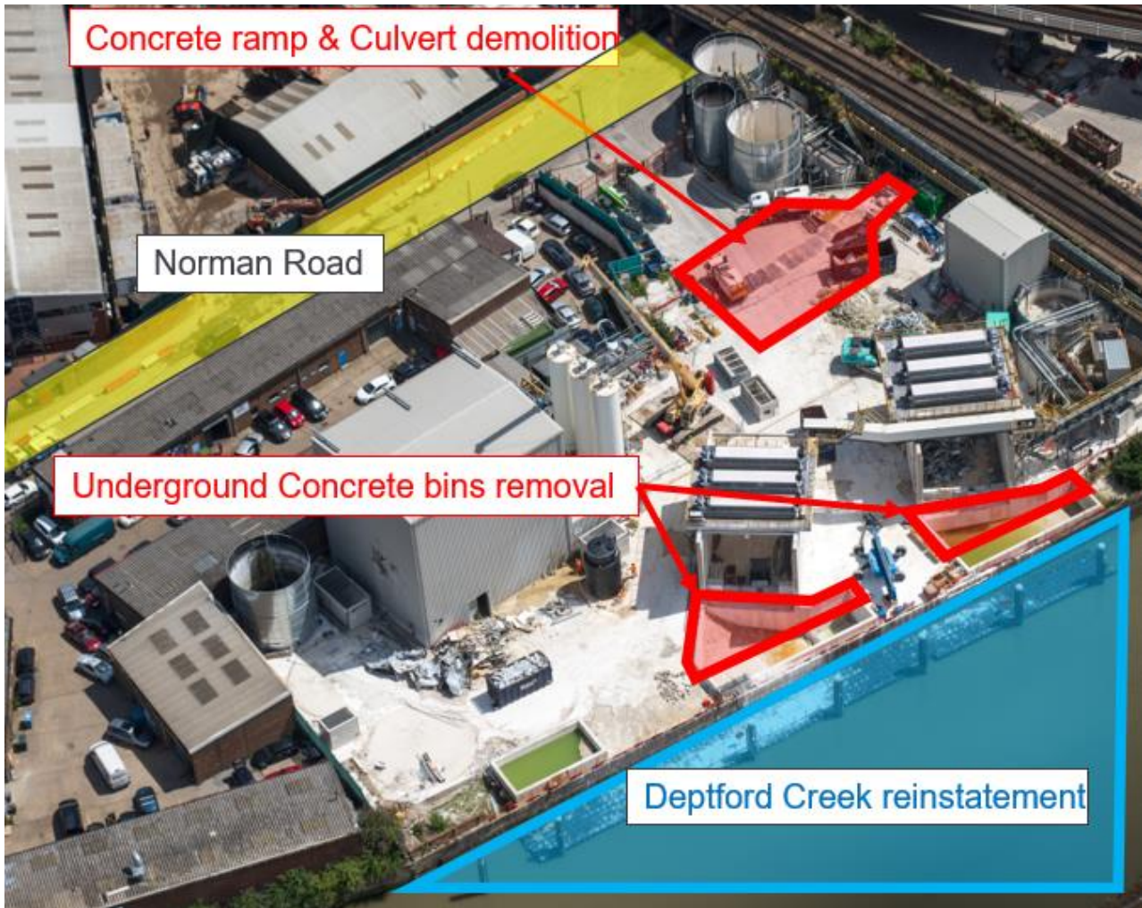
Aerial view of Phoenix Wharf, showing the service culvert, concrete ramp and below ground concrete storage bins to be removed
