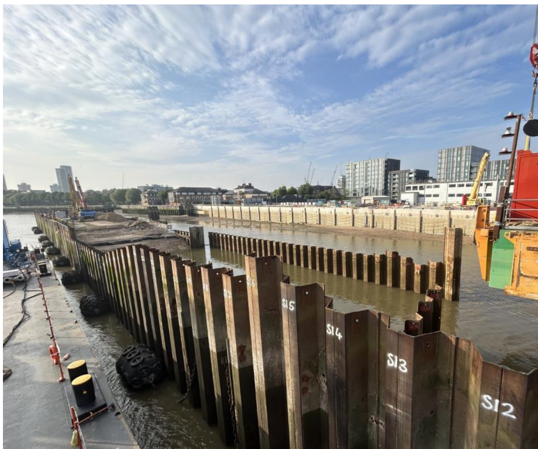
Picture shows the cofferdam 'island' remaining off Chambers Wharf
